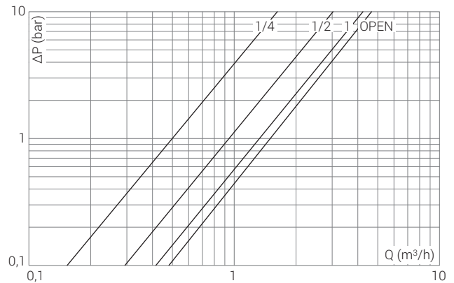
0393 0391 Valvole via dritta Straight radiator valves
