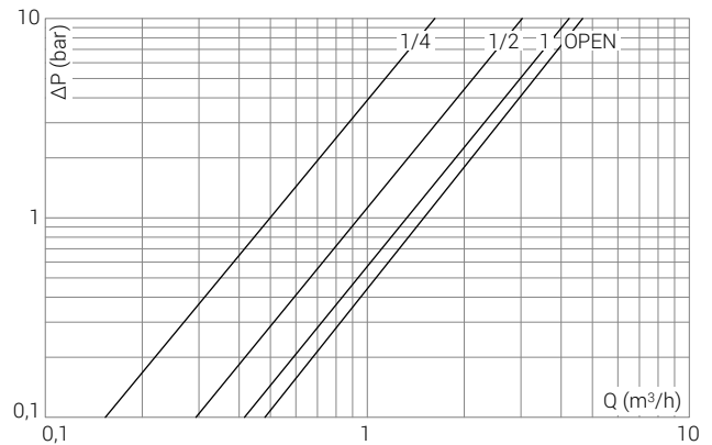
0319 0311 Valvole via dritta Straight radiator valves
